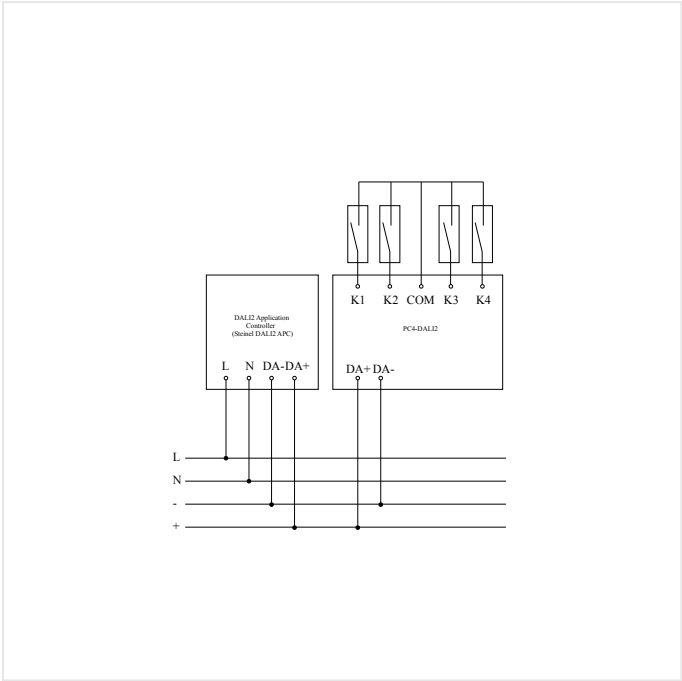
Connection of 4-fold push-button coupler to DALI2 APC
