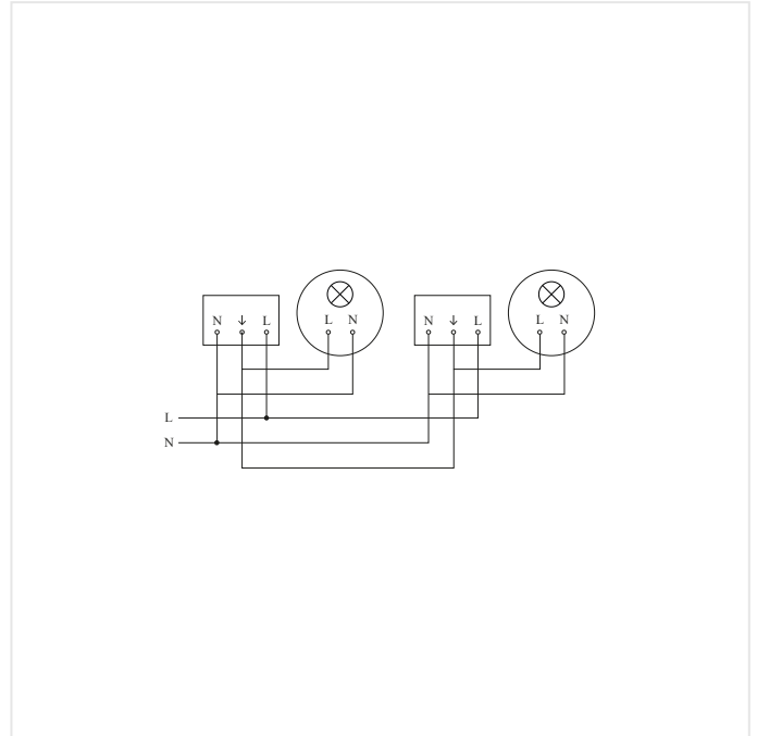
Master/slave interconnection circuit diagram
