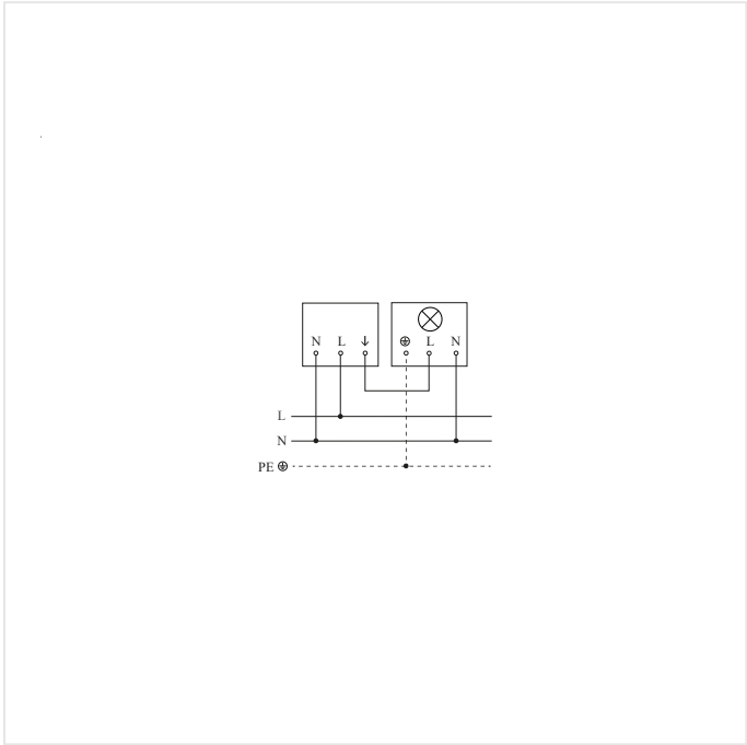
Master circuit diagram with switched luminaire
