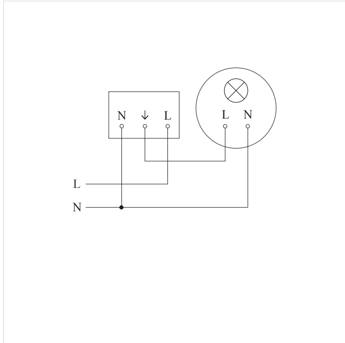
Circuit diagram
