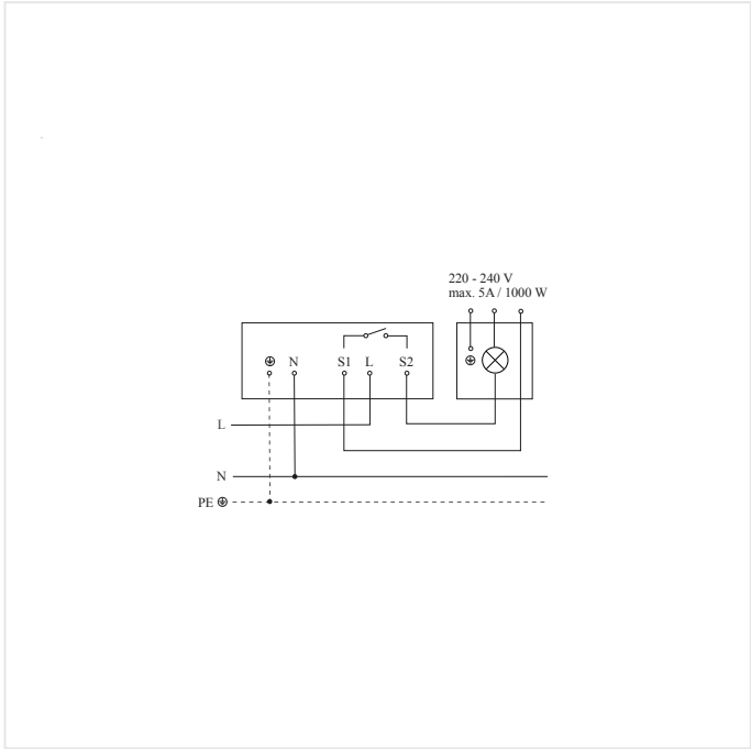
Master circuit diagram PF
